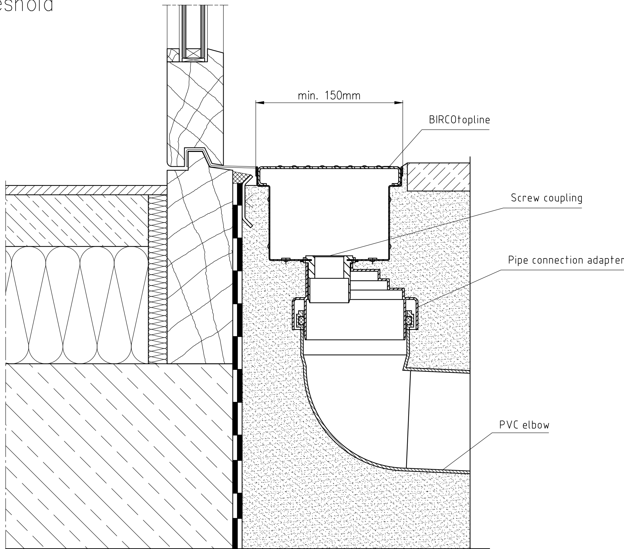
Door threshold – drainage via vertical connection without threshold
