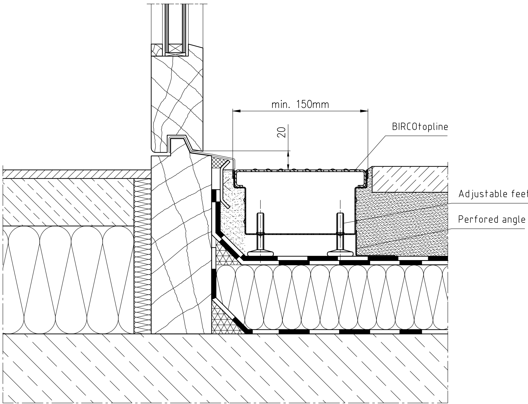
Door threshold – 20mm threshold
