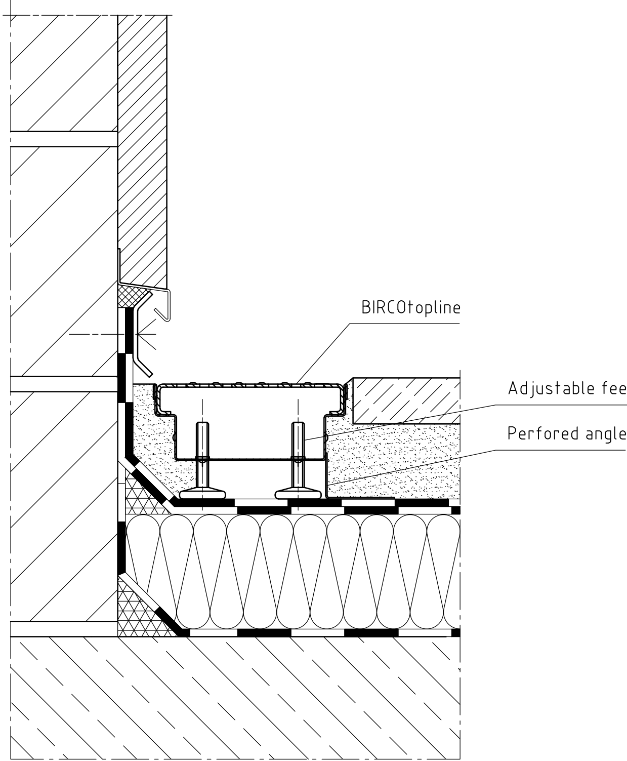
Facade support
