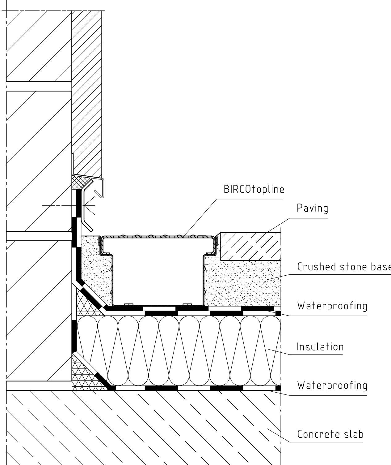
Door threshold – drainage via vertical connection without threshold
