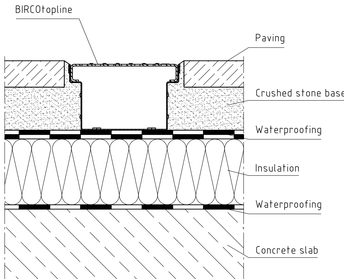
Paving – drainage without connection
