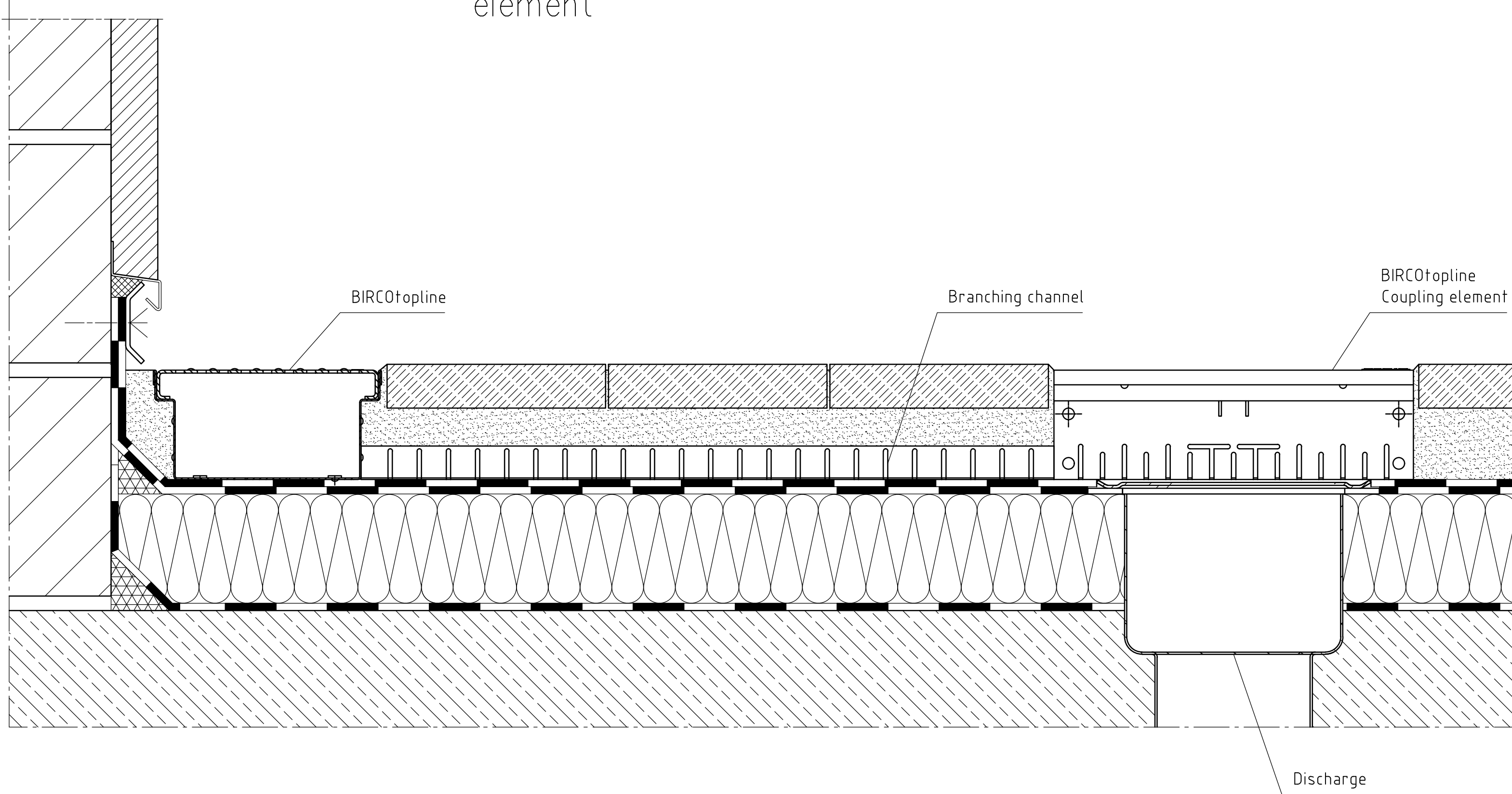
Facade support in combination with a connecting element
