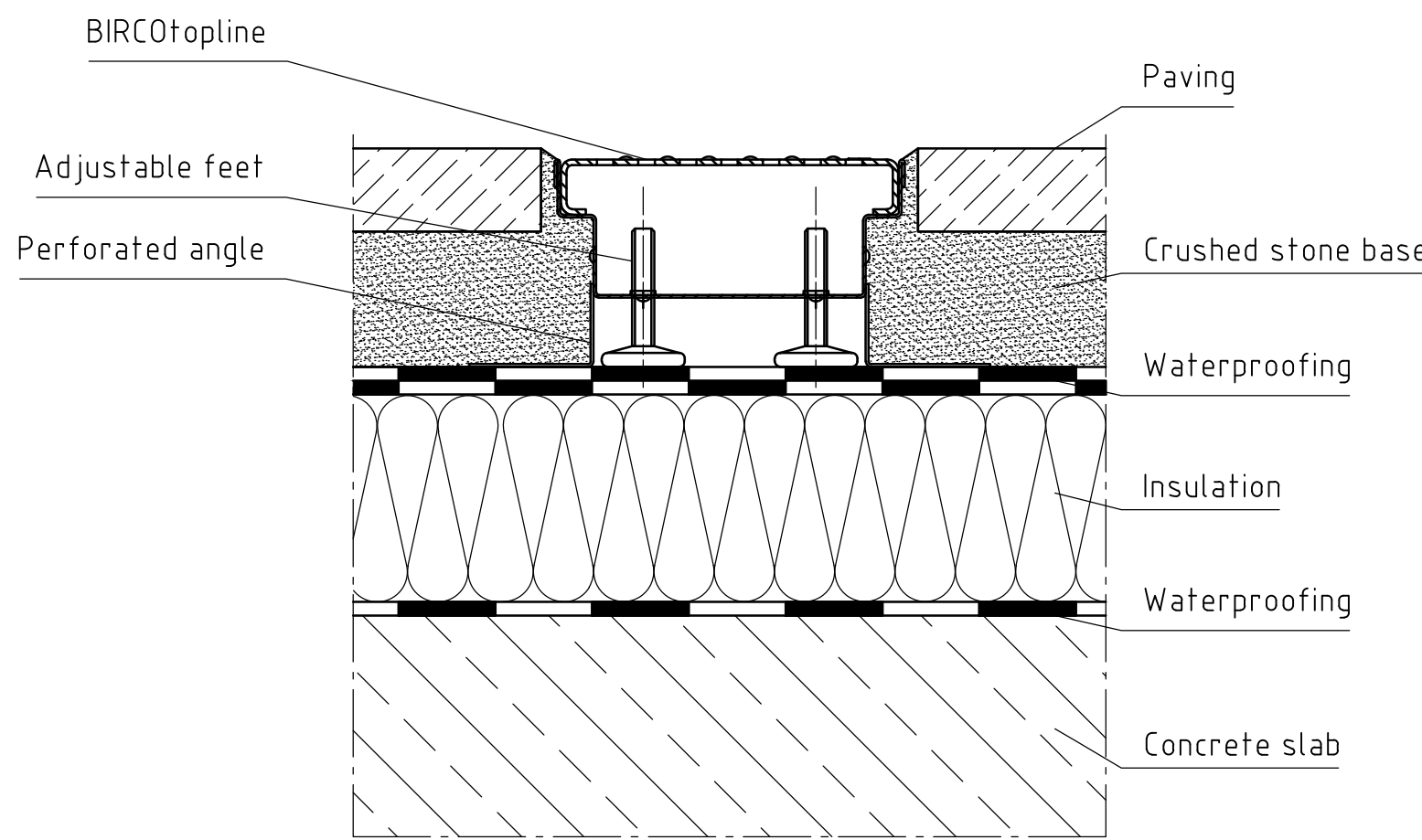
Paving – drainage without connection
